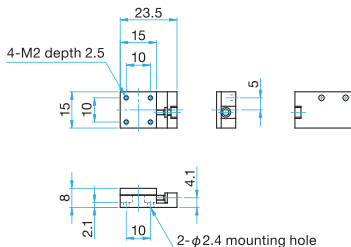
MLT11-15 Pan head screw M2×4...2 screws 2.5mm
