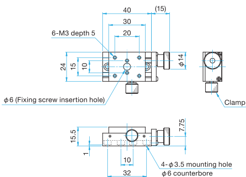
MLT11-2430 Pan head screw M3×5...4 screws
