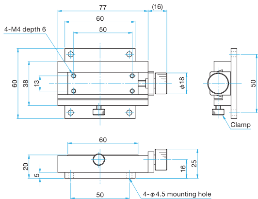
MLT11-2060 Hexagonal socket head cap screw M4×10...4 screws
