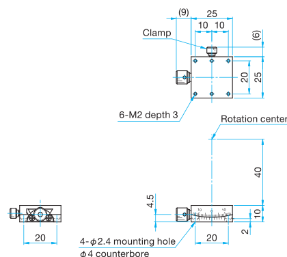
MGT11-25-40R Pan head screw M2x4...4 screws 2.5mm
