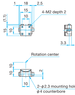
MGT11-15-10 Pan head screw M2x5...2 screws 2.5mm
