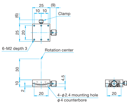
MGT11-25-30 Pan head screw M2x4...4 screws 2.5mm
