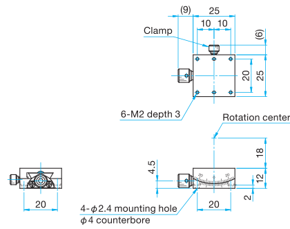
MGT11-25-18R Pan head screw M2x4...4 screws 2.5mm
