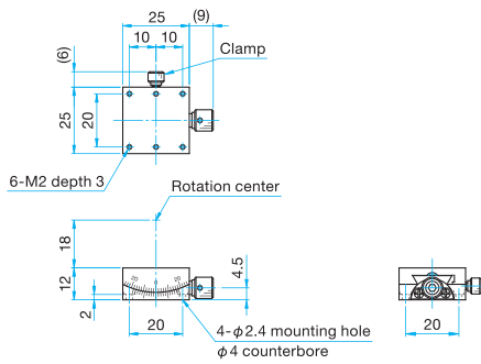
MGT11-25-18 Pan head screw M2x4...4 screws 2.5mm
