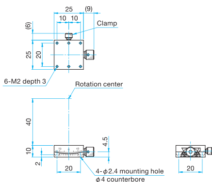
MGT11-25-40 Pan head screw M2x4...4 screws 2.5mm
