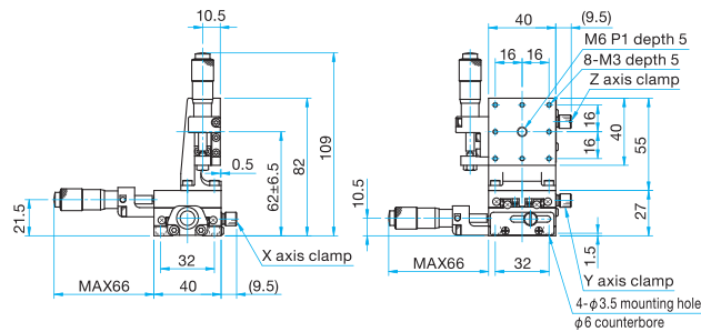
MLT35-40CL Pan head screw M3x6...4 screws, Spring washers
