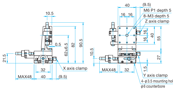
MLT35-40CLFP Pan head screw M3x6...4 screws, Spring washers 3mm
