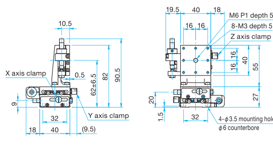
MLT35-40SLFP Pan head screw M3x6...4 screws, Spring washers 3mm
