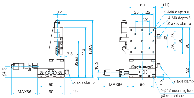
MLT35-60CL Hexagonal socket head cap screw M4x6...4 screws
