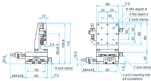
MLT35-60CLFP Hexagonal socket head cap screw M4x6...4 screws 3mm
