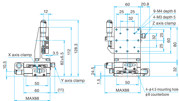
MLT35-60SL Hexagonal socket head cap screw M4x6...4 screws
