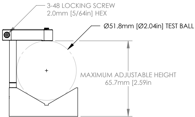
MAXIMUM CLAMPING HEIGHT
