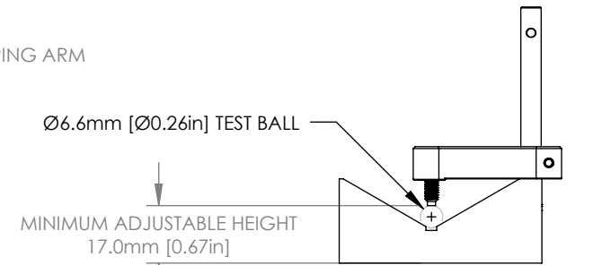
MINIMUM CLAMPING HEIGHT
