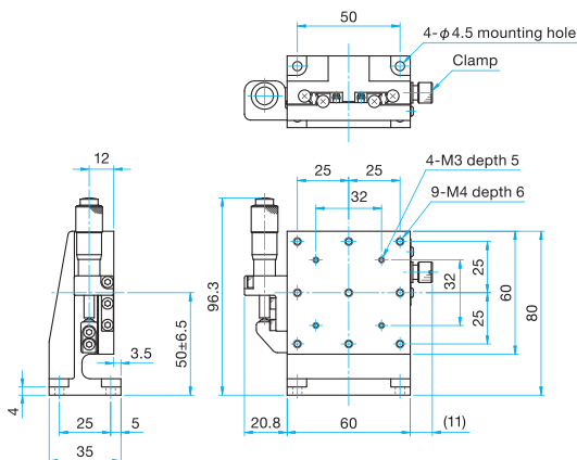
MLT33-60L Hexagonal socket head cap screw M4x8...4 screws
