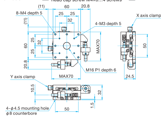
MLT32-60SWP Hexagonal socket head cap screw M4x6...4 screws
