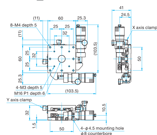
MLT32-60SWP Hexagonal socket head cap screw M4x6...4 screws
