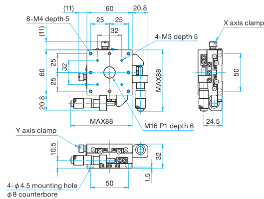
MLT32-60SR Hexagonal socket head cap screw M4x6...4 screws
