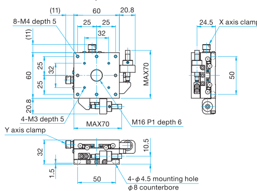
MLT32-60SDM Hexagonal socket head cap screw M4x6...4 screws
