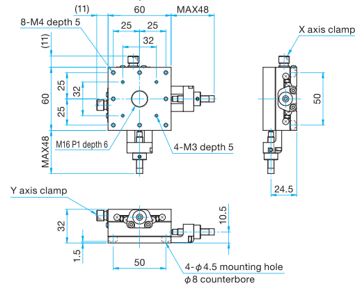
MLT32-60SR Hexagonal socket head cap screw M4x6...4 screws
