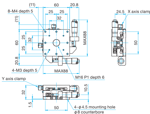
MLT32-60S Hexagonal socket head cap screw M4x6...4 screws
