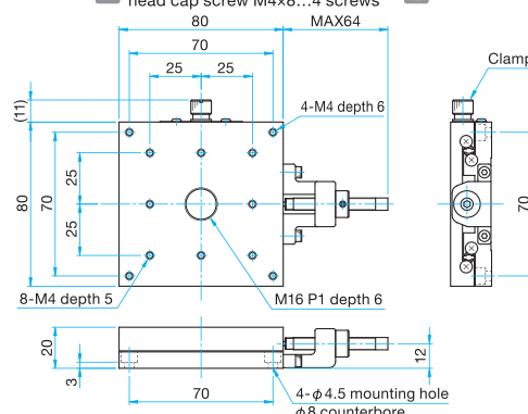
MLT31-80SR Hexagonal socket head cap screw M4x8...4 screws
