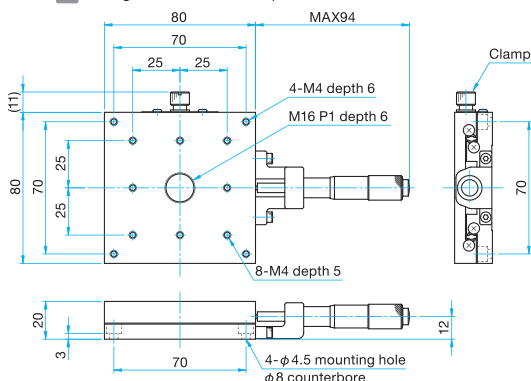
MLT31-80S Hexagonal socket head cap screw M4x8...4 screws
