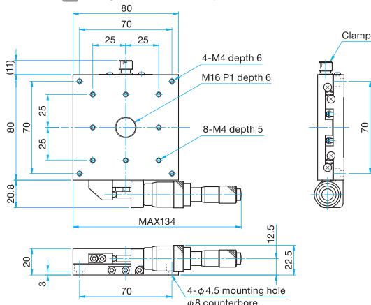
MLT31-80SDM Hexagonal socket head cap screw M4x8...4 screws
