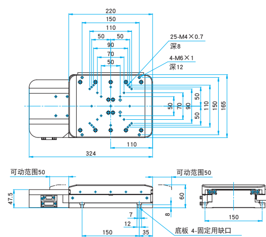
HST(GS)-100X-0B 内六角螺栓 M6×15...4个
