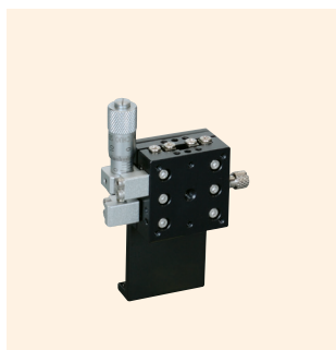
↑ LZ-3047-SR1
