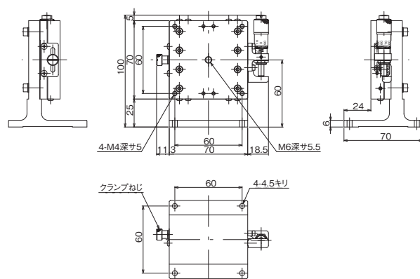
↑ LZ-7047-S8
